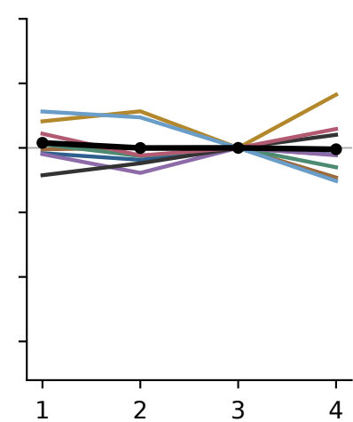
GAT layers
