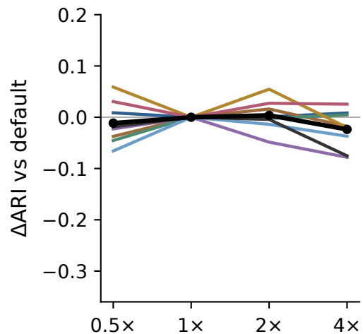
\lambda_{\text{cons}}
