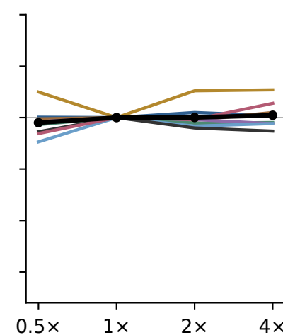
\lambda_{\text{bal}}
