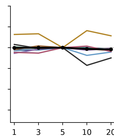
Prototypes R
