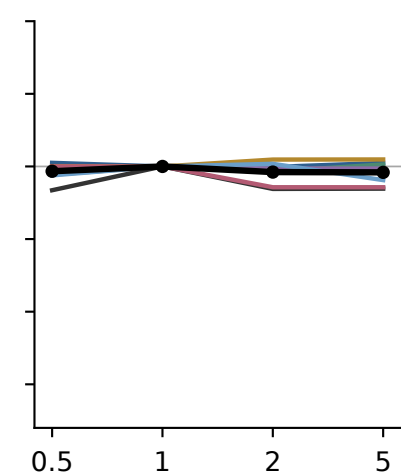
Student-t \alpha
