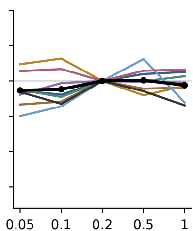
\tau_m
